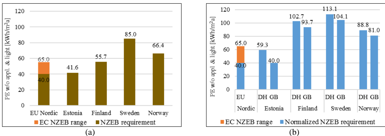
Fig. 5 National NZEB requirements directly compared with EC recommendation a), and national input data and primary energy normalized national NZEB requirements, b). Estonian TRY climate file was used for all countries in b) as a reasonable climate normalization within the same climatic zone.
