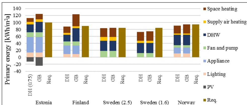
Fig. 4 PE in NZEB apartment buildings with changed technical solutions aiming to close compliance with national NZEB requirement.
